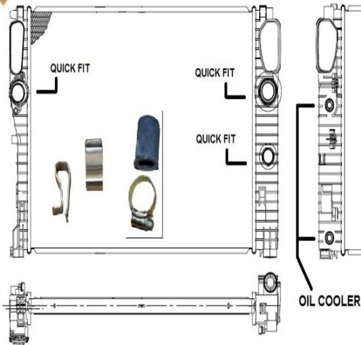
BACK-VIEW
